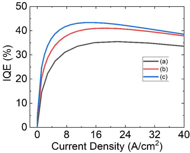
Fig. 3. IQE vs Current Density
