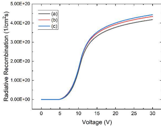
Fig. 4. Radiative Recombination Rate vs Voltage
