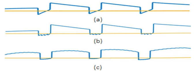
Fig. 2 (ii). Conduction band diagrams of reference and engineered active regions at a current density of 12 \text{ A/cm}^2
