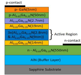
Fig. 1. Device Structure
