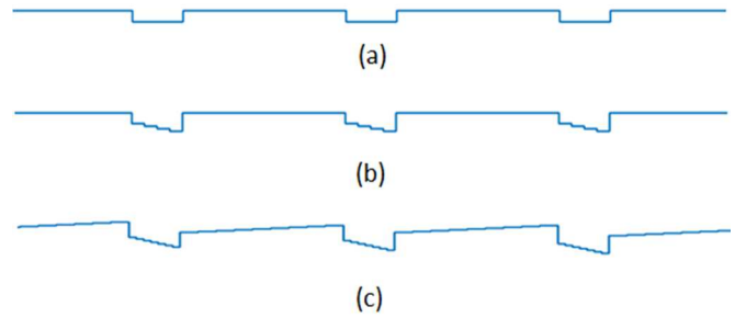
Fig. 2 (i). Reference and engineered conduction band profiles in active region
