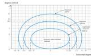
Fig.1. Diagram of isocandels of side lights at a runway width of 45 m (White lights)
