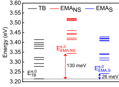
Fig. 1. The ten energetically lowest electron states (averaged over 10 alloy configurations) in an \text{In}_{0.1}\text{Ga}_{0.9}\text{N}/\text{GaN} QW. Tight-binding results in black, single-band effective mass approximation, with and without a shift of the conduction band edge energy, are given in blue and red, respectively.
