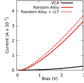
Fig. 2. Current voltage characteristics of a unipolar single \text{In}_{0.1}\text{Ga}_{0.9}\text{N} QW device. The calculations have been performed using a virtual crystal approximation (VCA, solid black) and when accounting for random alloy fluctuations. In the random alloy case, results with (dotted red) and without (solid red) quantum corrections via localization landscape theory are presented.
