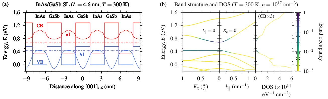
Fig. 1. (a) CB (red) and VB (blue) offsets, and electron (red) and hole (blue) ground state probability densities, for several periods of an InAs/GaSb SL having equal InAs and GaSb layer thickness t = 2.3 nm (SL period L = 4.6 nm). The dash-dotted red (blue) line shows the calculated electron (hole) ground state energy. (b) SL miniband structure (left-hand panel), in-plane band dispersion (centre panel), and density of states (DOS; right-hand panel) for the InAs/GaSb SL of (a). Line colours in (b) are weighted by Fermi-Dirac electron or hole occupancy, for temperature T = 300 K and carrier density n = 10^{17} cm ^{-3} .
