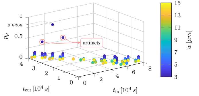
Fig. 3. Pseudo probability measure p_p depending on all primary and secondary process parameters t_{in} , t_{out} , w and c_0 . Numerical compression artifacts are marked.
