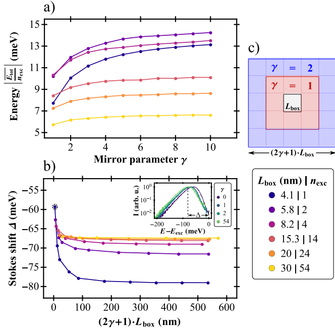
Fig. 1. a) The magnitude of the average mirror energy per exciton \overline{E_{\text{tot}}}/n_{\text{exc}} is depicted for increasing \gamma values. Contributions in the original box ( j = k = 0 in (1)) are excluded. b) The Stokes shift \Delta as a function of the effective box length (2\gamma+1) \cdot L_{\text{box}} : The dashed, black circle denotes the case of independent excitons without Coulomb interaction. The inset shows the PL spectra for L_{\text{box}} = 4.1 nm. c) A visualization of the original simulation box (grey) and the first two mirror sets (red and blue). The total number of mirror boxes for \gamma > 0 is (2\gamma+1)^2 - 1 .
