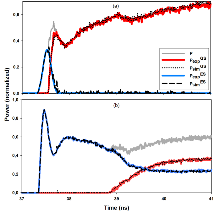
Fig. 1. ELM model time-response with (a) I = 123 \text{ mA} at 20^\circ\text{C} and (b) I = 174 \text{ mA} at 40^\circ\text{C} , where P is the QDL Optical Power; P_{exp}^{GS} and P_{sim}^{GS} are the Ground State Power, experimental and simulated, respectively; P_{exp}^{ES} and P_{sim}^{ES} are the Excited State Power, experimental and simulated, respectively.
