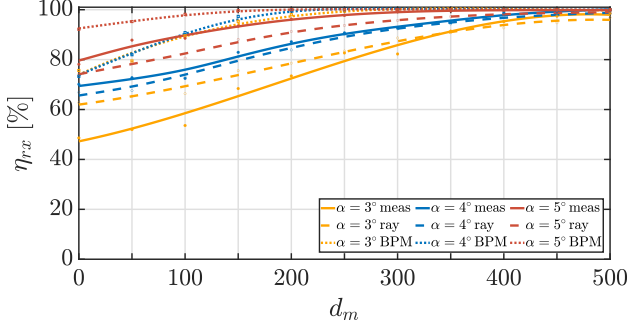
Fig. 2. Comparison of measured and calculated efficiencies \eta_{rx} in the receiving direction (RX) for various combinations of the mask bridge d_m and coupling angle \alpha .
