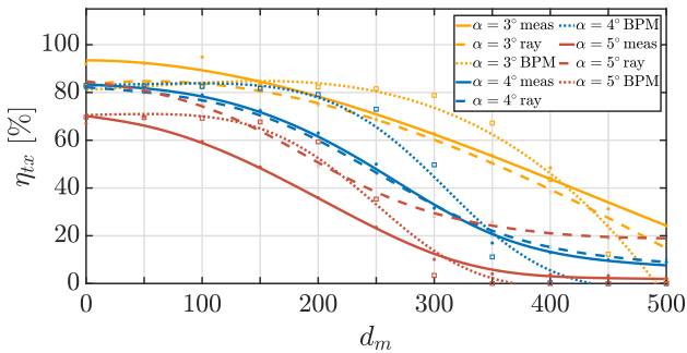
Fig. 3. Comparison of measured and calculated efficiencies \eta_{tx} in the transmission direction (TX) for various combinations of the mask bridge d_m and coupling angle \alpha .
