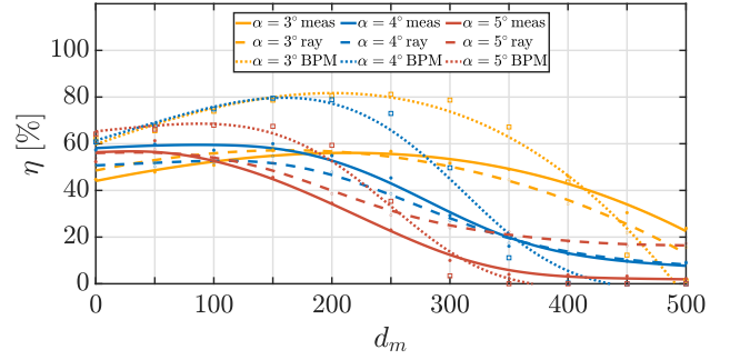
Fig. 4. Overall efficiency \eta for various combinations of the mask bridge d_m and coupling angle \alpha .
