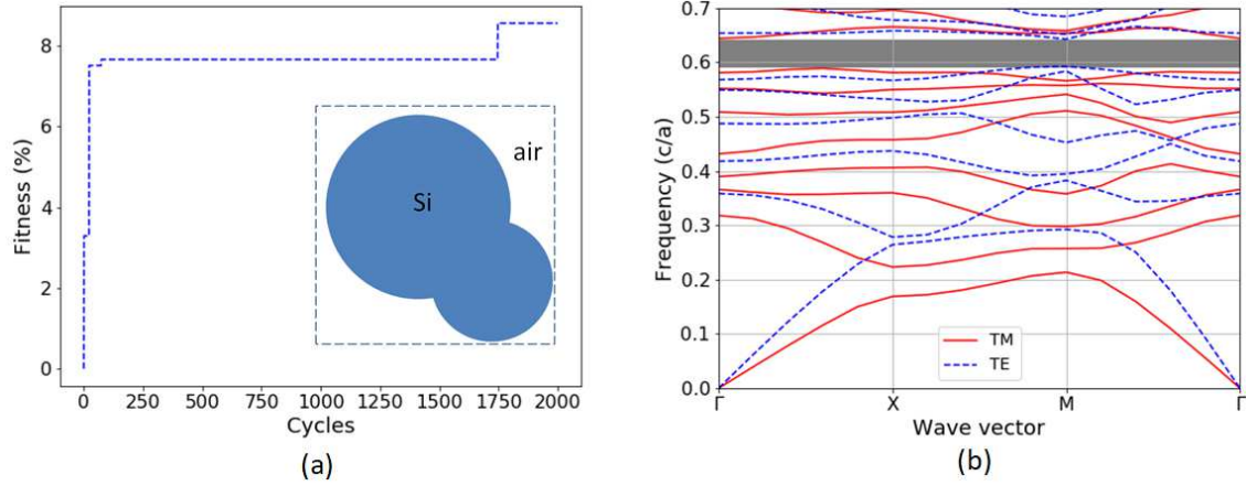
Fig. 1. a) Convergence curve of ABC algorithm. Inset shows the optimum unit cell obtained from the ABC code. b) Diagram band of the unit cell in a).
