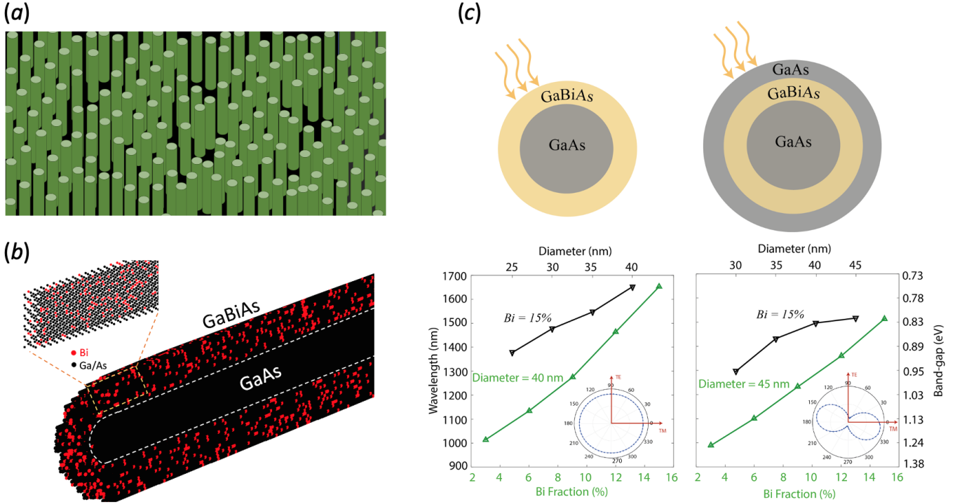
Fig. 1. (a) Schematic diagram of an array of vertical nanowires. (b) One \text{GaBi}_x\text{As}_{1-x}/\text{GaAs} nanowire is zoomed in to indicate atomistic structural construction in which Bi atoms randomly replace As atoms in the GaAs shell region. (c) (Top Row) Schematic diagram of investigated \text{GaBi}_x\text{As}_{1-x}/\text{GaAs} and \text{GaAs}/\text{GaBi}_x\text{As}_{1-x}/\text{GaAs} nanowires shown. (Bottom Row) Absorption wavelength is plotted as a function of the nanowire shell diameter (at 15% and Bi fraction (at 40 nm or 45 nm diameter). (Insets) The insets show polarisation dependent optical transition spectra.
