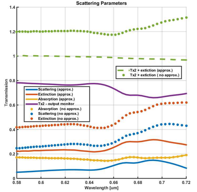
Figure 3: Simulation results after Scattering Theory processing.
