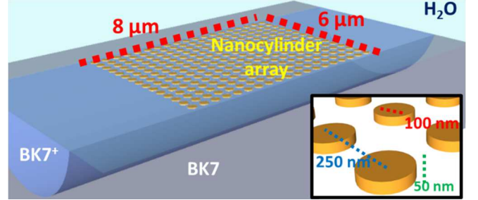
Figure 1: Schematic view of the structure under analysis. The inset shows the details of the nano-array.
