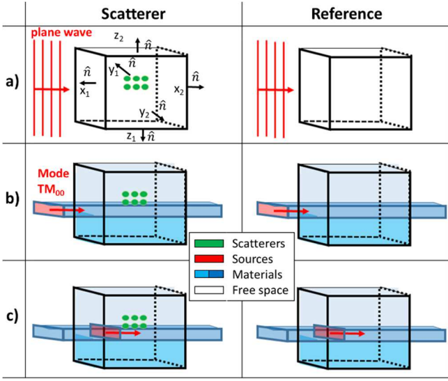
Figure 2: Setup approaches in terms of monitor box and source type: (a) classical configuration, (b) waveguide with source outside the box, (c) waveguide with source inside box.
