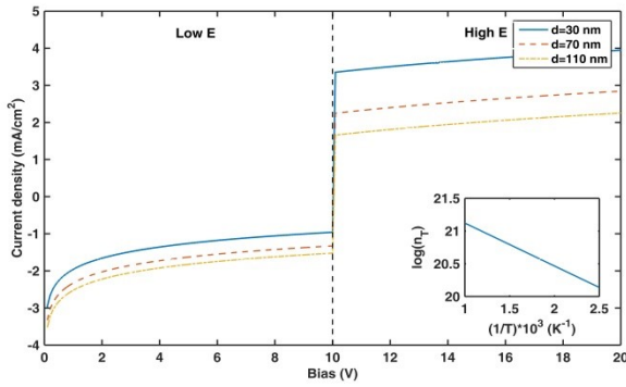
Fig. 1. Current density for varying bias at different QD layer thickness and no. of free charge carriers as function of inverse temperature (inset)
