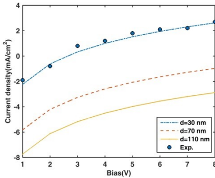
Fig. 2. Current density for varying bias at different QD layer thickness in presence of traps
