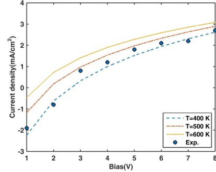
Fig. 3. Current density for varying bias at different temperatures in presence of traps
