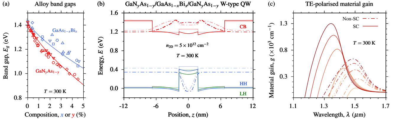
Fig. 1. (a) Calculated (lines) and measured (symbols) band gap vs. composition for \text{GaAs}_{1-x}\text{Bi}_x (blue) and \text{GaN}_y\text{As}_{1-y} (red) alloys grown pseudomorphically on (001) GaAs. (b) Band offsets of an exemplar strain-balanced 1.55 \mu\text{m} \text{GaN}_y\text{As}_{1-y}/\text{GaAs}_{1-x}\text{Bi}_x/\text{GaN}_y\text{As}_{1-y} W-type QW having band offset ratio \Delta E_{VB} = 2 \Delta E_{CB} , in the absence of injected carriers (light colours) and at an injected carrier density n_{2D} = 5 \times 10^{12} \text{ cm}^{-2} (full colours). (c) Non-self-consistent (dashed lines) and self-consistent (solid lines) calculated optical gain spectra at n_{2D} = 2, 4, 6, 8 and 10 \times 10^{12} \text{ cm}^{-2} (darkening colours) for the W-type QW of (b).
