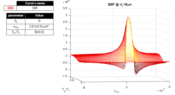
Fig. 5. SDF at \delta_1 = 0 .
