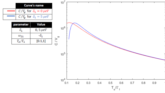
Fig. 2. Group speed Miniaturization up to 6 order of magnitude compared to normal light speed in logarithmic diagram.
