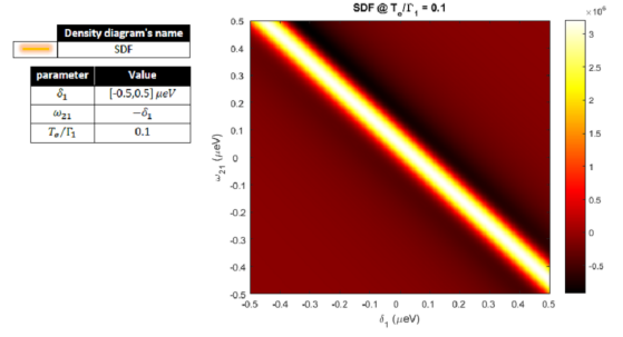
Fig. 4. SDF at T_e = \Gamma_1/10 .
