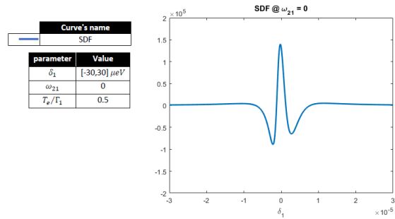
Fig. 3. SDF at \omega_{21} = 0 and T_e = \Gamma_1/2 .
