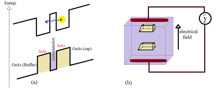
Fig. 1. (a) The direction of the electric force caused by the applied electric field will lead to the energy level of the electric carrier tilt in the quantum structure. (b) The cross-section of our QD structure.
