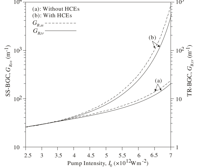
Fig. 2. Variation of SS and TR BGCs with pump intensity at n_0 = 2 \times 10^{19} \text{ m}^{-3} .
