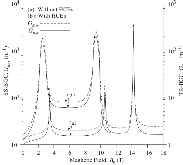
Fig. 1. Variation of SS and TR BGCs with external magnetic field at n_0 = 2 \times 10^{19} \text{ m}^{-3} , I_0 = 6.5 \times 10^{12} \text{ Wm}^{-2} .
