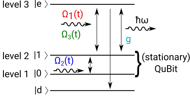
Fig. 1. Level scheme for entangling a stationary Qubit with a photon in a time bin realization.
