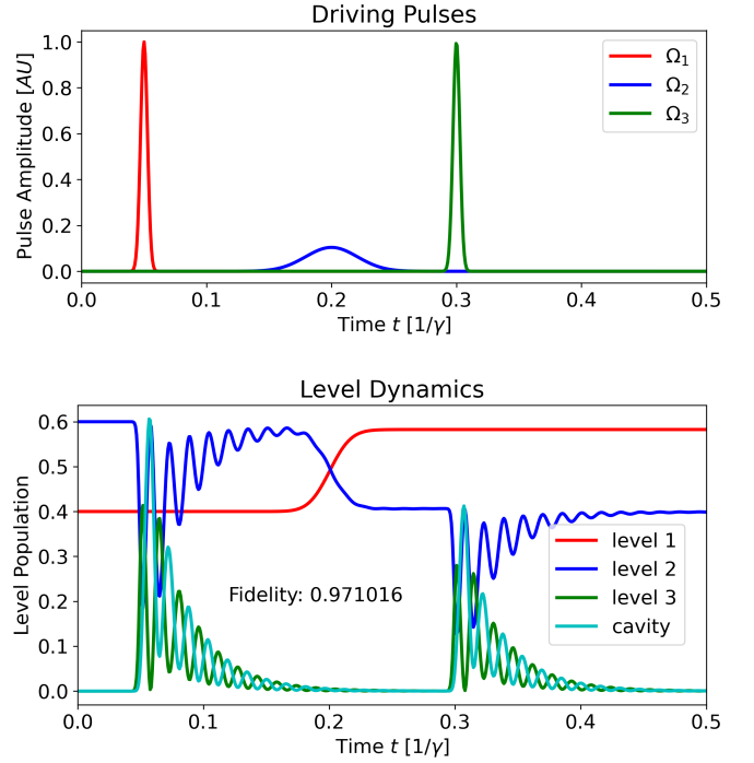
Fig. 2. Top: Pulse sequence. \Omega_1 and \Omega_3 drive the optical transition, \Omega_2 flips the Qubit. Bottom: Population dynamics for optimized pulses for mixed Qubit starting condition.
