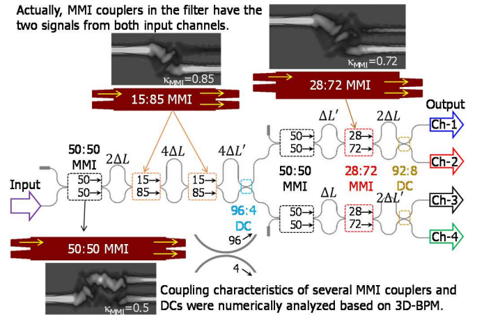
Fig. 1. Proposed MDI-type wavelength filters for Coarse WDM applications.
