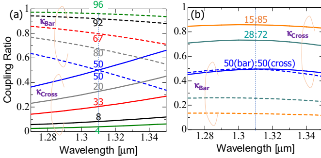
Fig. 2. Calculated \kappa for (a)DCs and (b)MMI couplers for flat filter spectra.
