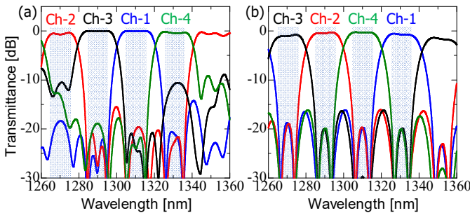
Fig. 3. Calculated CWDM spectra based on (a)DCs and (b)proposed scheme.
