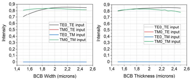
Fig. 4: Fiber-to-chip coupling efficiency in terms of BCB waveguide width and thickness
