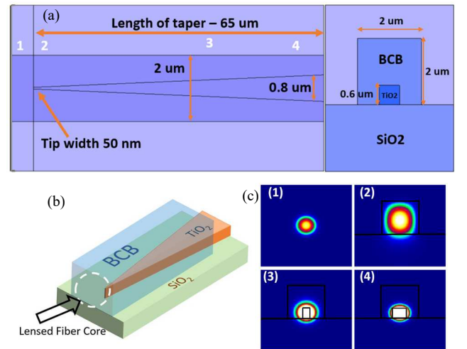
Fig. 1: (a) top view and cross section of the spot size converter with the tapered TiO 2 waveguide buried in BCB waveguide, (b) layout of the inverse adiabatic taper coupler, and (c) mode evaluation of the inverse taper
