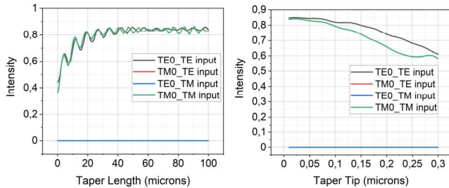
Fig. 3: Fiber-to-chip coupling efficiency in terms of taper length and taper tip variation from the proposed designed parameters
