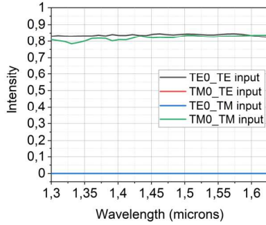
Fig. 2: Fiber-to-chip coupling efficiency in terms of wavelengths for the proposed designed parameters
