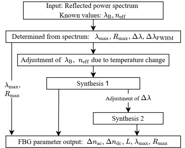
Fig. 1. Flow chart of the implemented FBG synthesis. The FBG parameters needed for the Digital Shadow are the output values.
