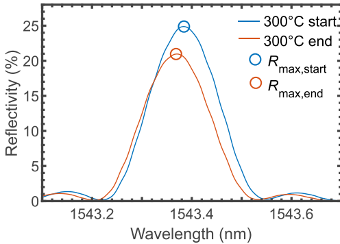
Fig. 2. Measured spectra at the beginning of the aging process (blue curve) and after 168 hours at 300 °C (red curve). The maximum reflectivity decreases 3.9%. Also, a slight left shift of 15.9 pm of the maximum wavelength is visible.
