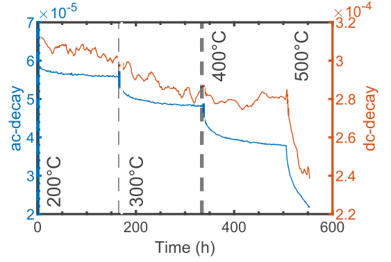
Fig. 3. Thermal decay of ac- and dc-refractive index change over the whole aging process from 200 °C to 500 °C. With the beginning of each temperature step, a drop in ac-index change \Delta n_{\text{ac}} is visible.
