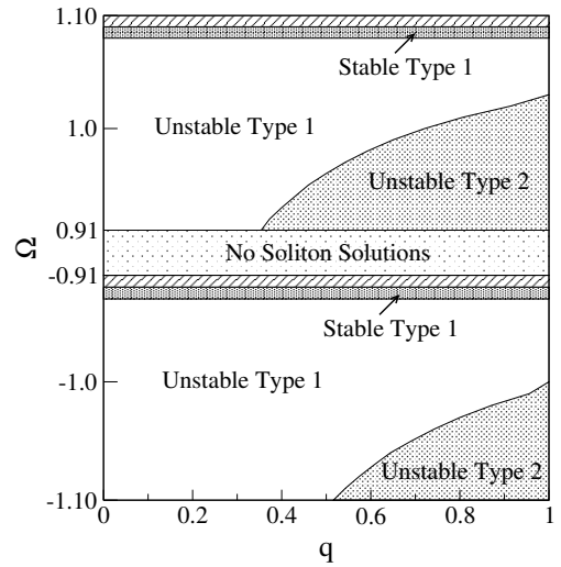
Fig. 3. Stability diagram for moving soliton corresponding to \sigma = 0.2 , \lambda = 0.2 and c = 0.2 on the (q, \Omega) plane.
