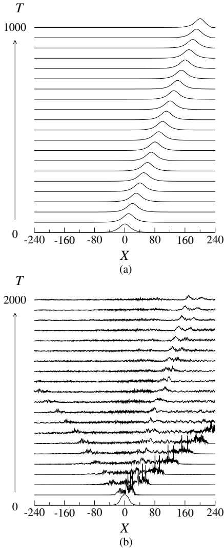
Fig. 2. Propagation of solitons with \lambda = 0.2 , c = 0.2 and \sigma = 0.2 showing: (a) stable Type 1 soliton for \Omega = 1.09 , q = 0.26 ; (b) unstable Type 2 soliton for \Omega = -1.05 , q = 0.7 .
