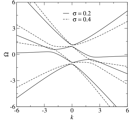
Fig. 1. Linear spectra for different velocities at \lambda = 0.2 and c = 0.2 .
