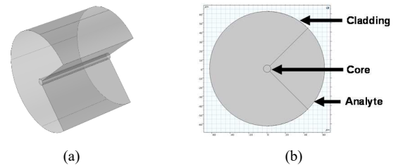
Fig. 1. The structure of C – shaped OFS in a) 3D and b) cross section geometry for simulation purposes
