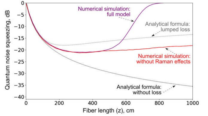
Fig. 1. Kerr squeezing of CW light in tellurite fibers: numerically simulated in the framework of the full model described by Eq. (1); numerically simulated in the framework of Eq. (1) without Raman effects; analytically estimated without loss and Raman effects using formula (2); and analytically estimated with lumped loss using formula (3).
