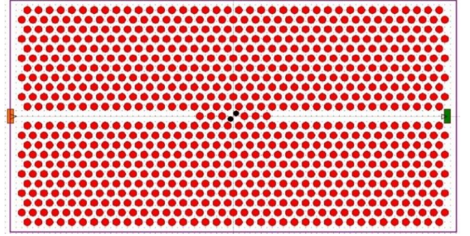
Fig.4. Schematic of the modified 2D-PhC biosensor.
