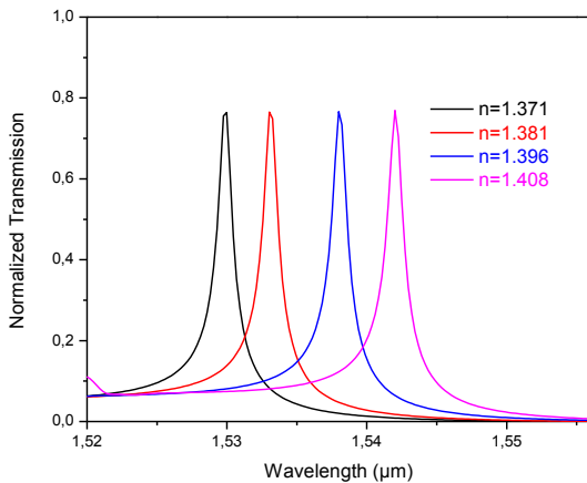
Fig.3. Normalized transmission spectrum for R=0.25 \times a .
