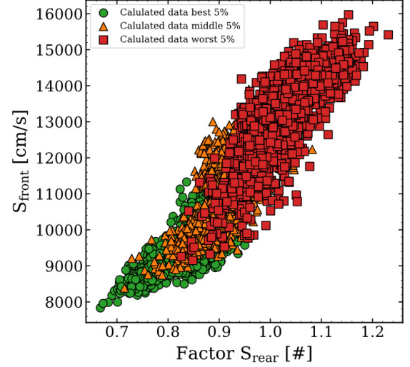
FIG. 3. Corresponding simulation input parameters to modelled data points in Figure 1, from machine learning, of the SRH recombination velocity at the front surface over the rear surface. Same colors as in Fig. 1.
