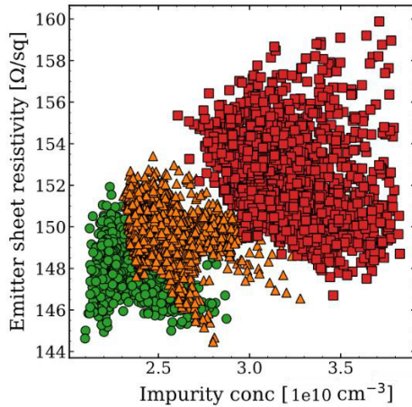
FIG. 2. Corresponding simulation input parameters to modelled data points in Figure 1, from machine learning, of the emitter sheet resistivity over the concentration of interstitial iron, limiting the excess carrier lifetime. Same colors as in Fig. 1.
