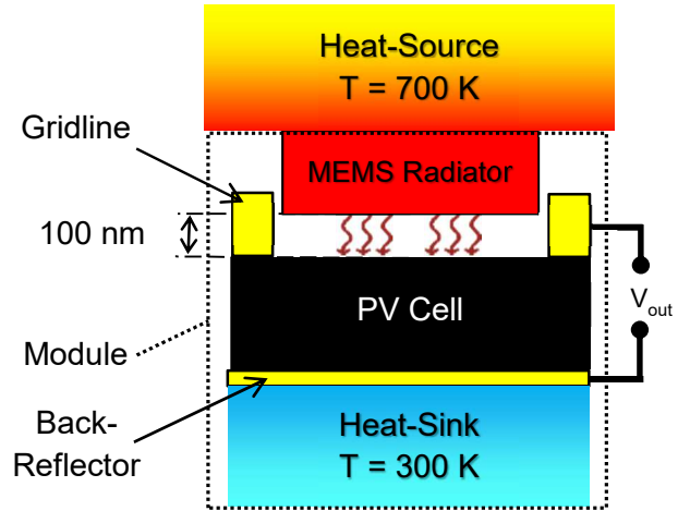
Figure 1 Schematic diagram of our proposed NFTPV module.
