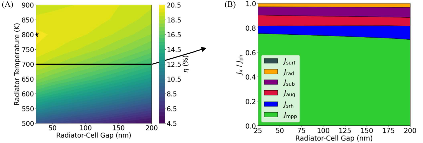
Figure 2 (A) Color plot of system efficiency as a function of radiator-cell separation and radiator temperature. The star represents the maximum calculated efficiency. (B) Currents, at maximum power point, normalized to the total generated current as a function of the radiator-cell separation for 700 K radiator.
