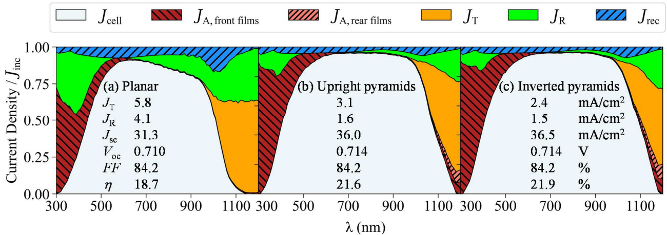
Fig. 3. Sources of current loss at P_{\text{max}} for normal-incidence front illumination with front and rear surface textures as labelled.
