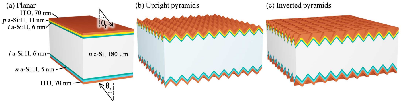
Fig. 1. Modelled bifacial SHJ cell structure with varied texturing (not to scale). Layer thicknesses are labelled. The AOI of incoming rays is pictured for front and rear illumination, given by \theta_f and \theta_r , respectively.
