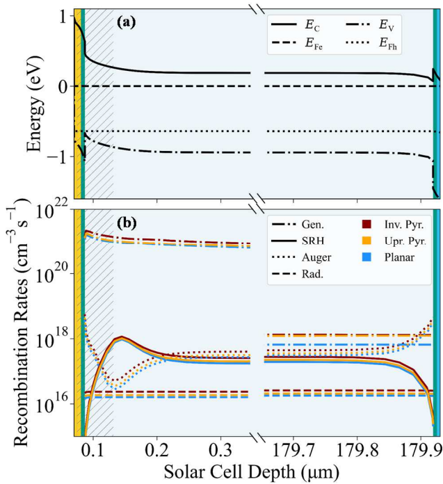
Fig. 2. (a) Electronic band structure and (b) generation and recombination rates for the bifacial SHJ under front illumination at P_{\text{max}} for varied textures.
