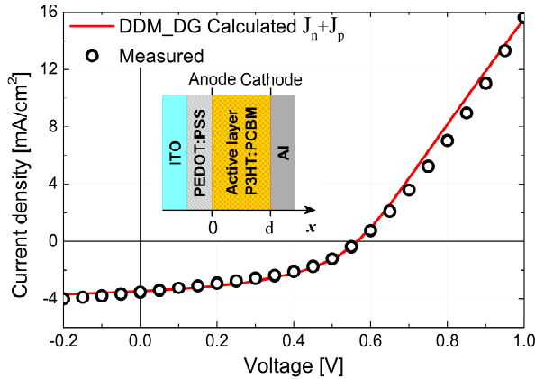
Fig 2. The ITO/PEDOT:PSS/P3HT:PCBM/Al solar cells J - V curves, measured and simulated by the DDM_DG model with Dirichlet BCs. Schematics of the device – Inset.
