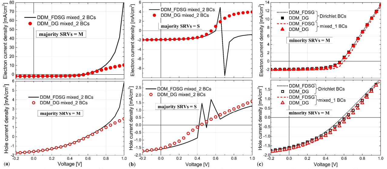
Fig.1. J_n - V and J_p - V curves simulated by DDM_FDSG and DDM_DG models for (a) mixed_2 BCs with M SRVs values, (b) mixed_2 BCs with S SRVs values, and (c) Dirichlet and mixed_1 BCs with M SRVs values.
