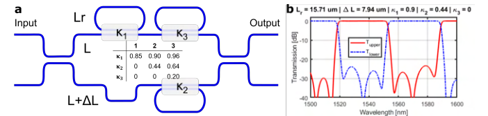
Fig. 1. a) Illustration of the analytical model for 3 basic RAMZI configurations, including 1, 2, and 3 assist rings. For each case, \kappa_i is the optical power coupling coefficient into each ring from the respective RAMZI arm, optimizing for flatness in the pass-band [4]. b) Analytically modeled output spectra of 2-ring configuration RAMZI with r_{ring} = 2.5\mu\text{m} and n_g = 4.35 . Band suppression ratio is 20+ dB and the functional dichroic bandwidth is 70+ nm. Filter roll-off, measured from the 3 dB point to 20 dB, is 7.8 dB/nm.
